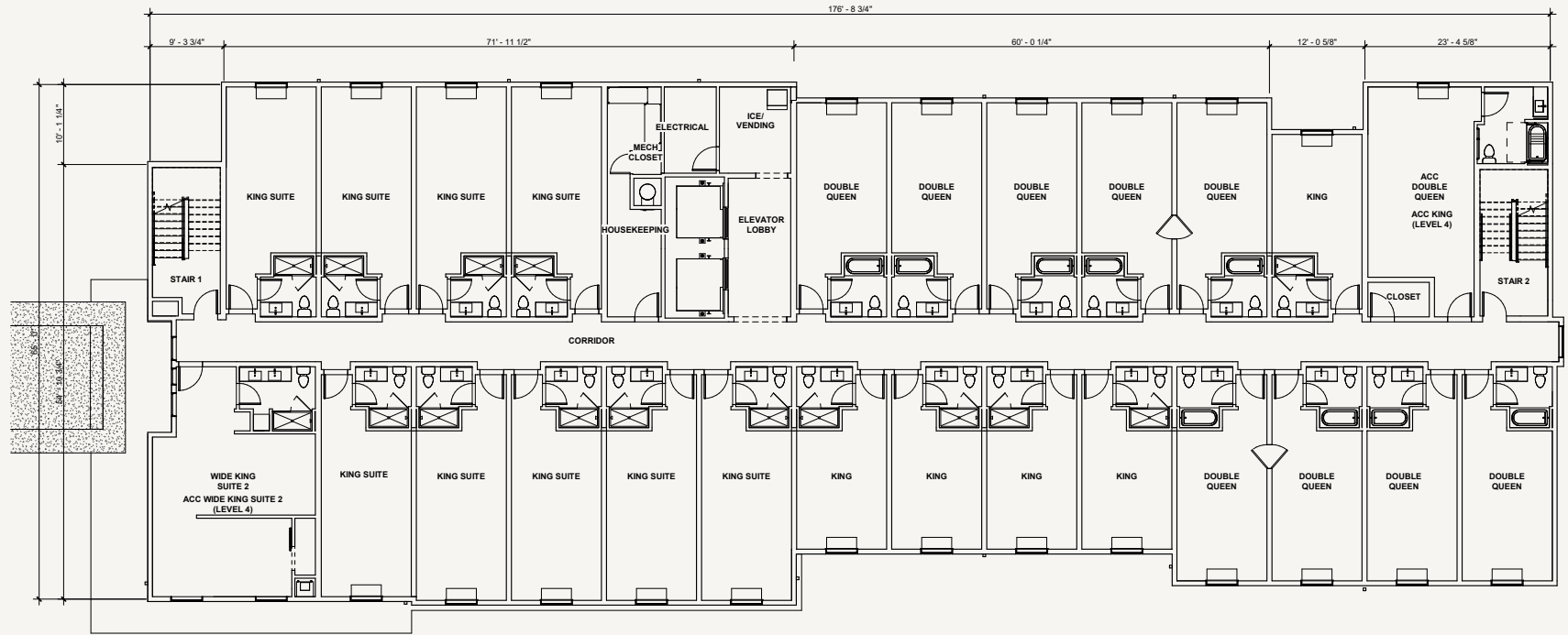
Typical Floorplan
